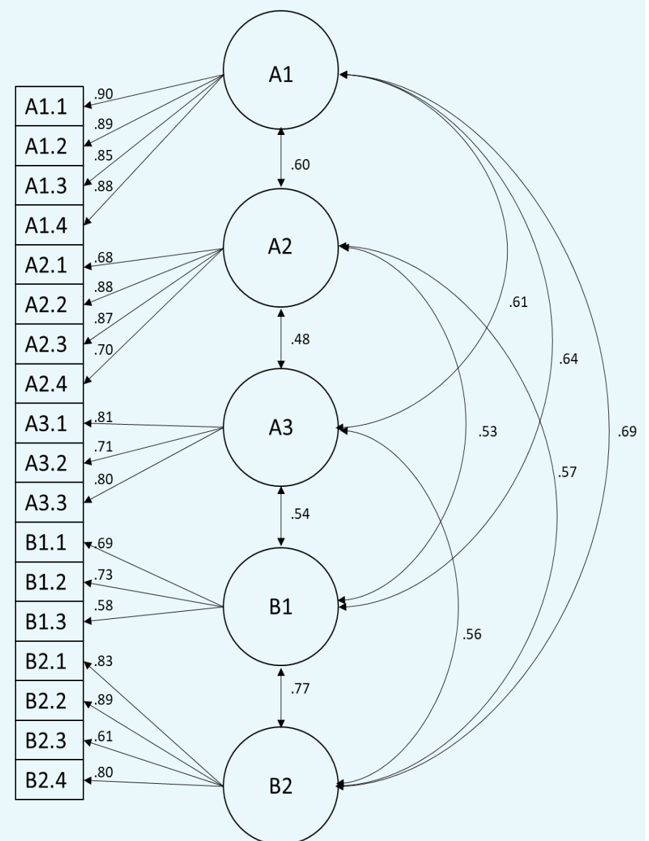
Figure 2 : Path diagram – population totale
